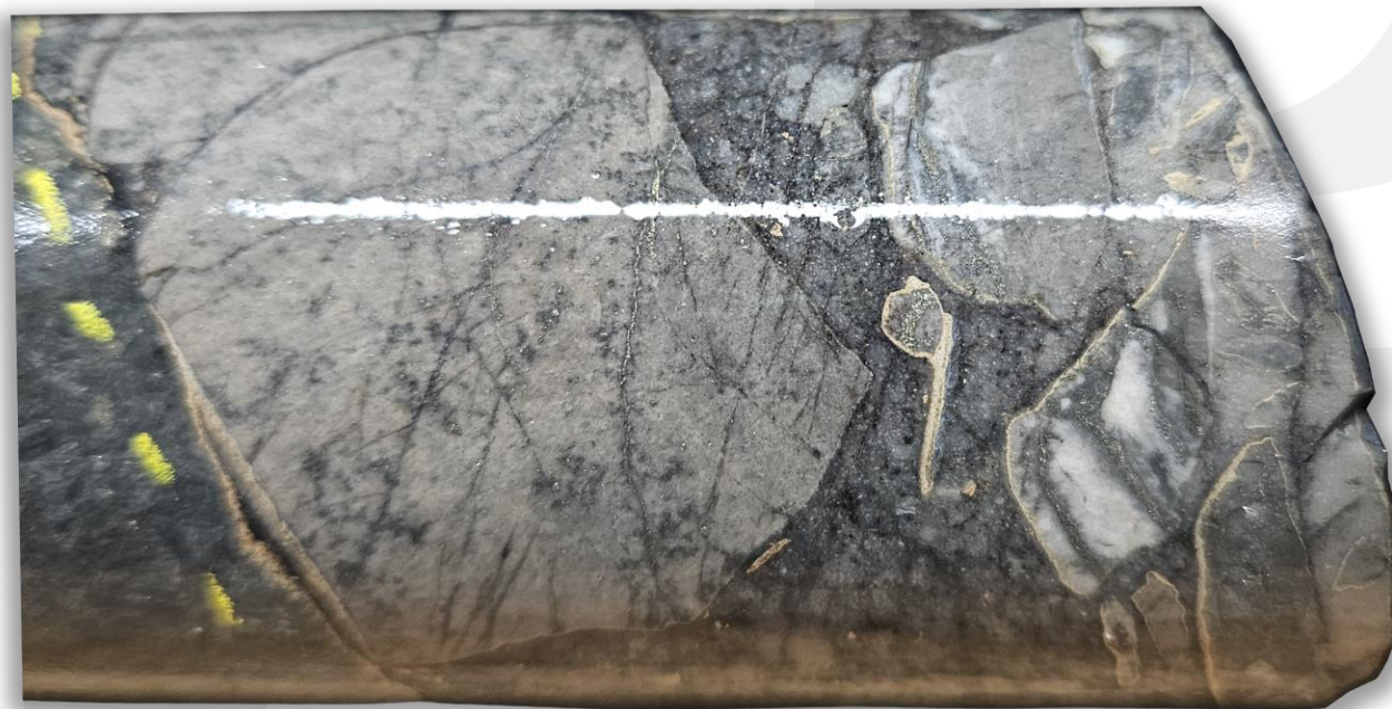
Porphyry intrusive breccia exhibiting strong silica-sericite-pyrite replacement – Cyprus Project 2025 drill core (DD25CYP003)
