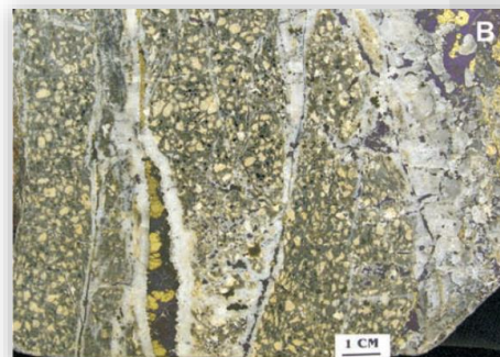
Quartz-bornite-chalcopyrite veins - Granisle Deposit
